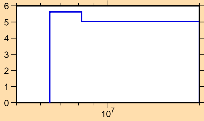
\Delta\sigma/\sigma vs. E for ^{174}\text{Ho}(n,\text{nonel.})
