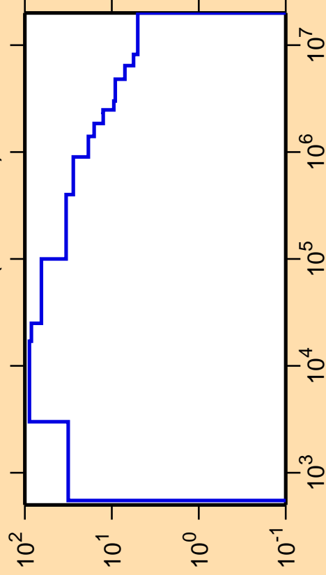
\Delta\sigma/\sigma vs. E for ^{174}\text{Ho}(n,\text{nonel.})
