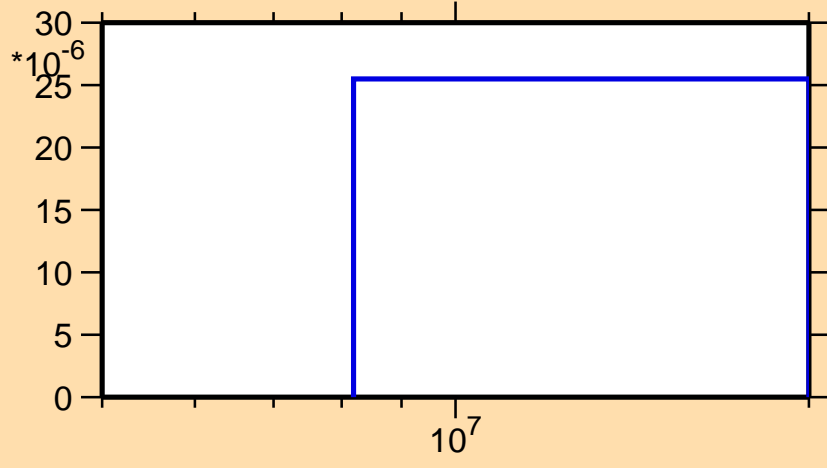
\sigma vs. E for ^{174}\text{Ho}(n,t)
