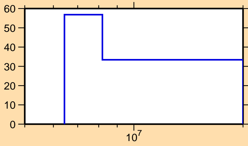
\Delta\sigma/\sigma vs. E for ^{174}\text{Ho}(n,\text{inel.})
