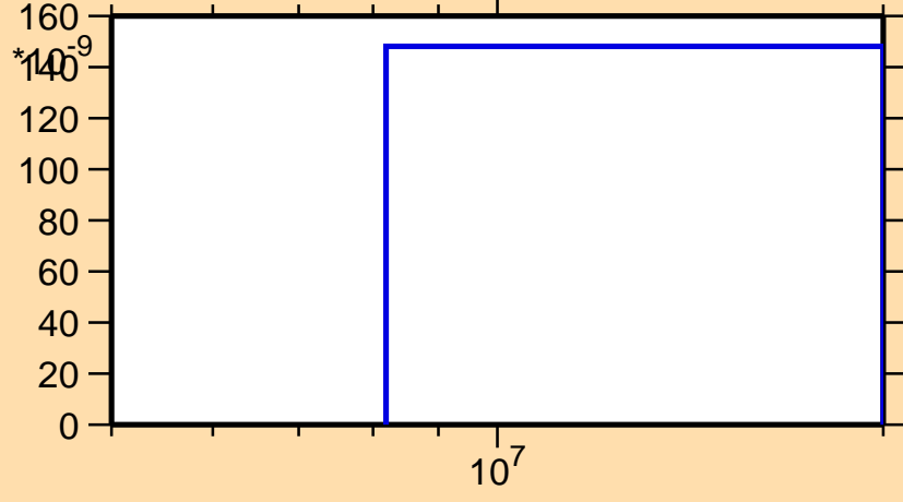
\sigma vs. E for ^{174}\text{Ho}(n,nt)
