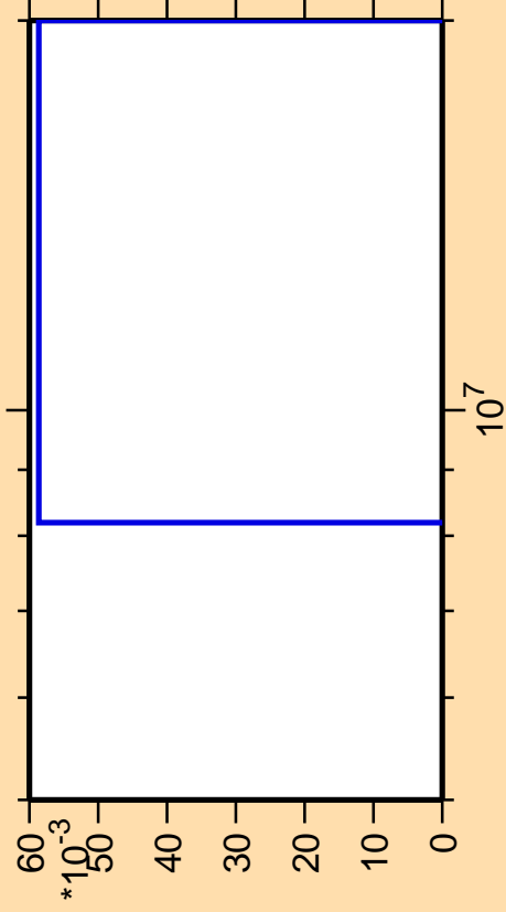
\Delta\sigma/\sigma vs. E for ^{174}\text{Ho}(n,3n\alpha)
