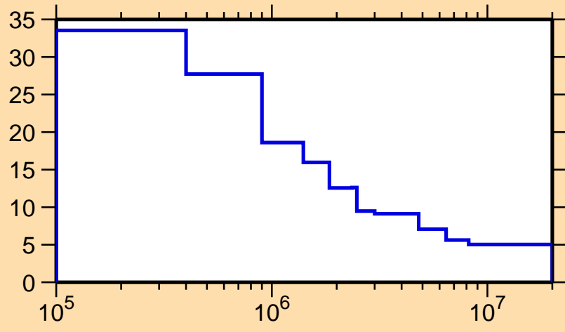
\Delta\sigma/\sigma vs. E for ^{174}\text{Ho}(n,\text{nonel.})
