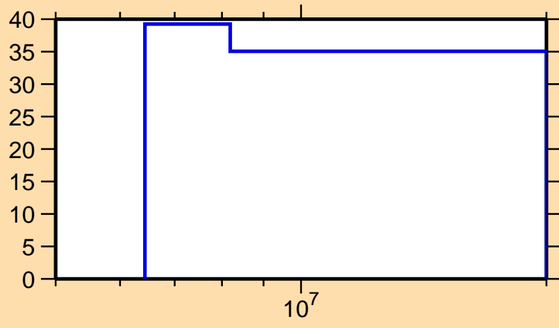
\Delta\sigma/\sigma vs. E for ^{174}\text{Ho}(n,n_1)
