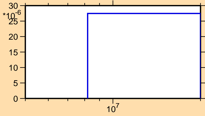
\sigma vs. E for ^{174}\text{Ho}(n,d)
