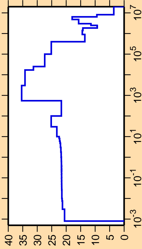
\Delta\sigma/\sigma vs. E for ^{174}\text{Ho}(n,\text{el.})
