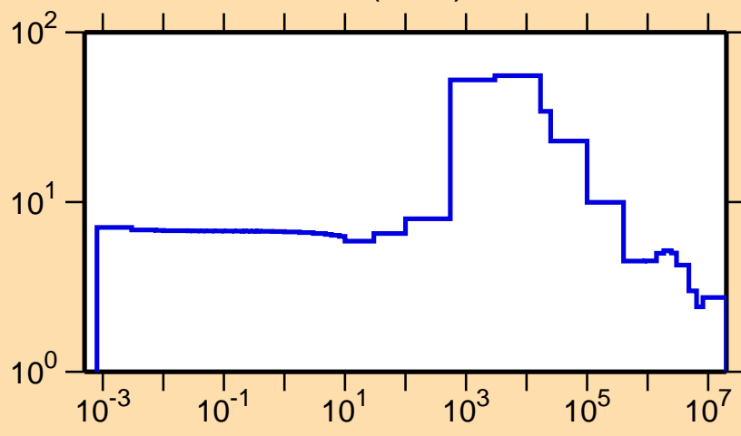
\sigma vs. E for ^{174}\text{Ho}(n,\text{el.})
