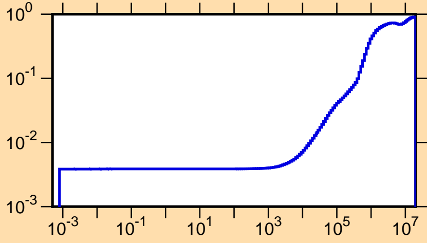
\mu vs. E for ^{175}\text{Ho}(\text{mt251})
