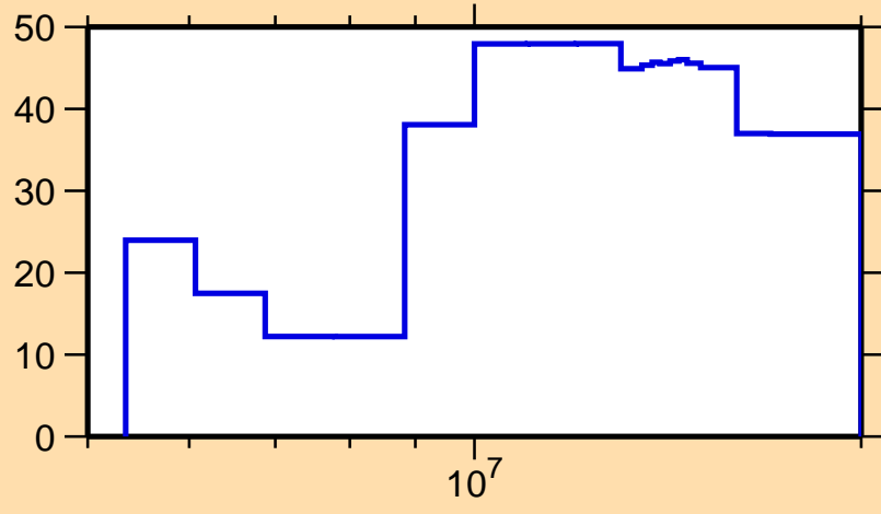
\Delta\sigma/\sigma vs. E for ^{175}\text{Ho}(n,2n)
