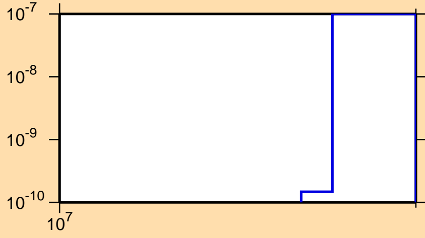
\sigma vs. E for ^{175}\text{Ho}(n,\text{nd})
