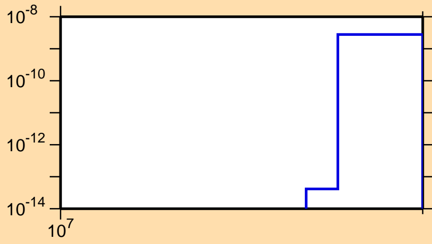
\sigma vs. E for ^{175}\text{Ho}(n,2np)
