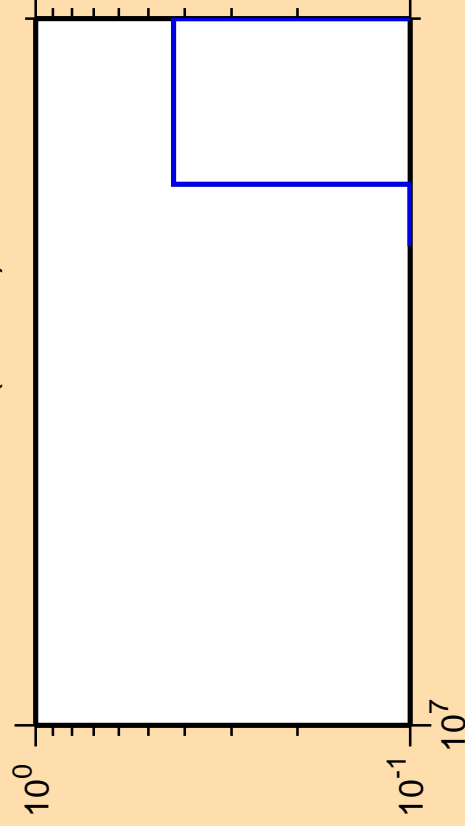
\Delta\sigma/\sigma vs. E for ^{175}\text{Ho}(n,3n\alpha)
