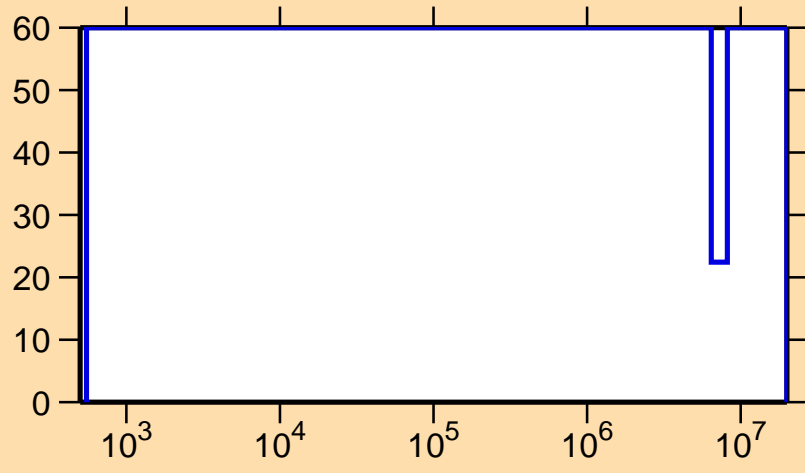
\Delta\sigma/\sigma vs. E for ^{268}\gamma
