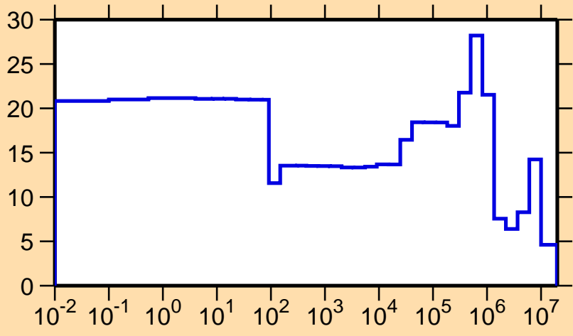
\Delta\sigma/\sigma vs. E for ^{269}\text{Pa}
