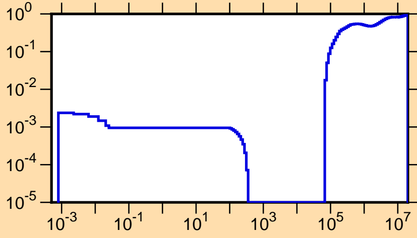
\mu vs. E for 272
