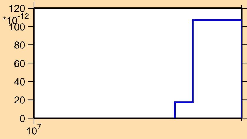
\sigma vs. E for ^{272}\text{He3}
