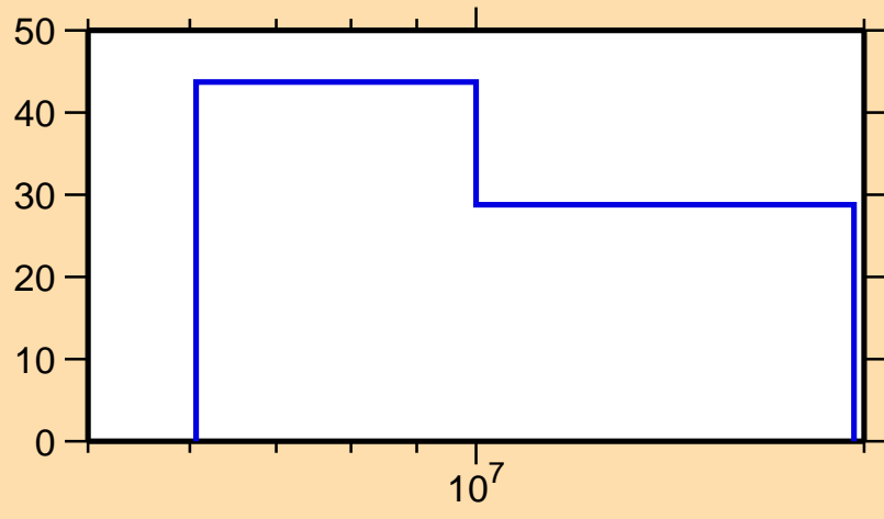
\Delta\sigma/\sigma vs. E for ^{272}\text{P}
