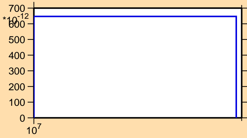
\sigma vs. E for ^{111}\text{I} (mt 34)
