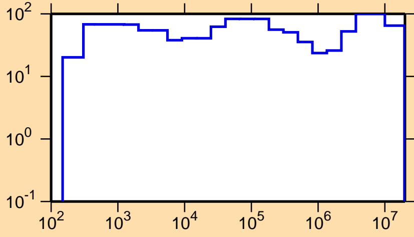
\Delta\sigma/\sigma vs. E for ^{111}\text{I}(n,p)
