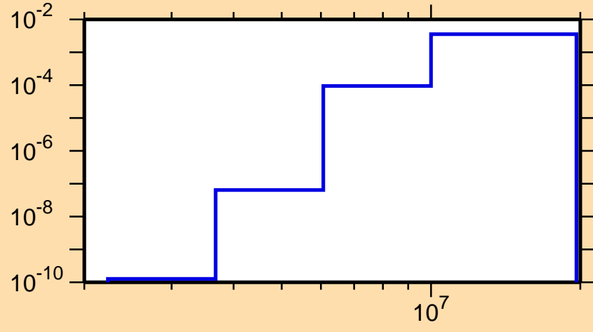
\sigma vs. E for ^{111}\text{I}(\text{mt117})
