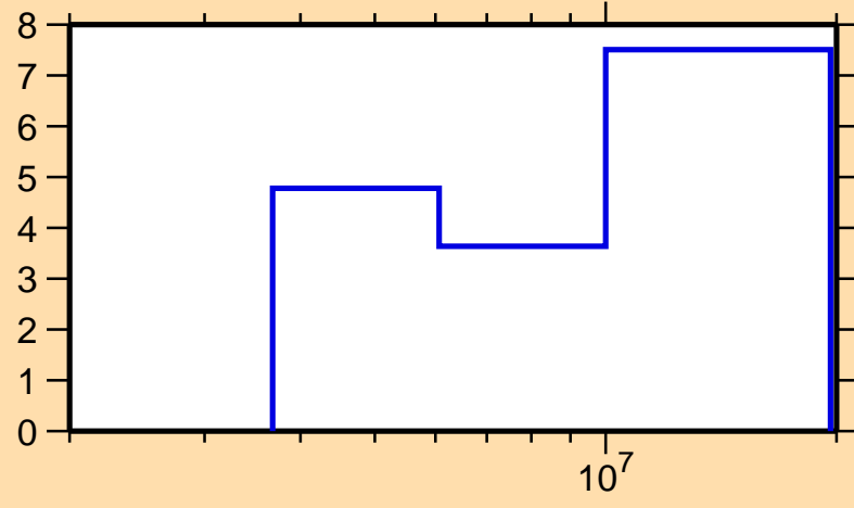
\Delta\sigma/\sigma vs. E for ^{111}\text{I}(n, tot.)
