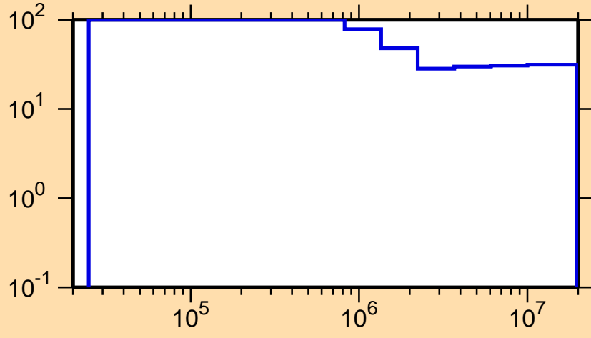
\Delta\sigma/\sigma vs. E for ^{111}\text{I}(n,n_1)
