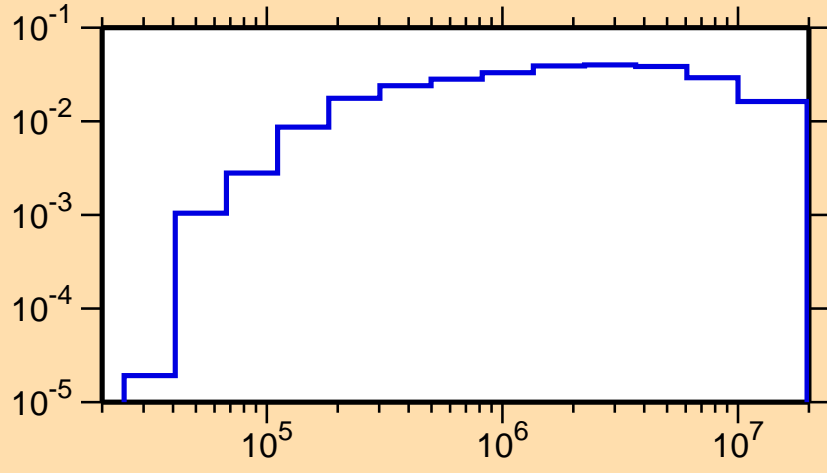
\sigma vs. E for ^{111}\text{I}(n,n_1)
