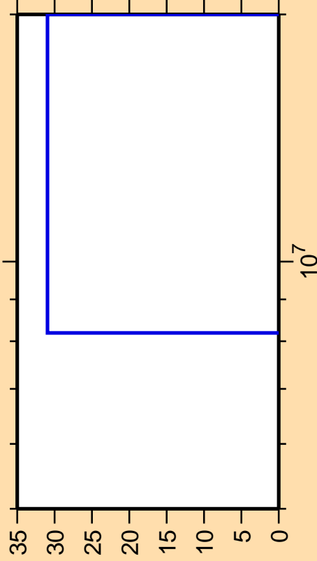
\Delta\sigma/\sigma vs. E for ^{111}\text{I}(n,n_1)
