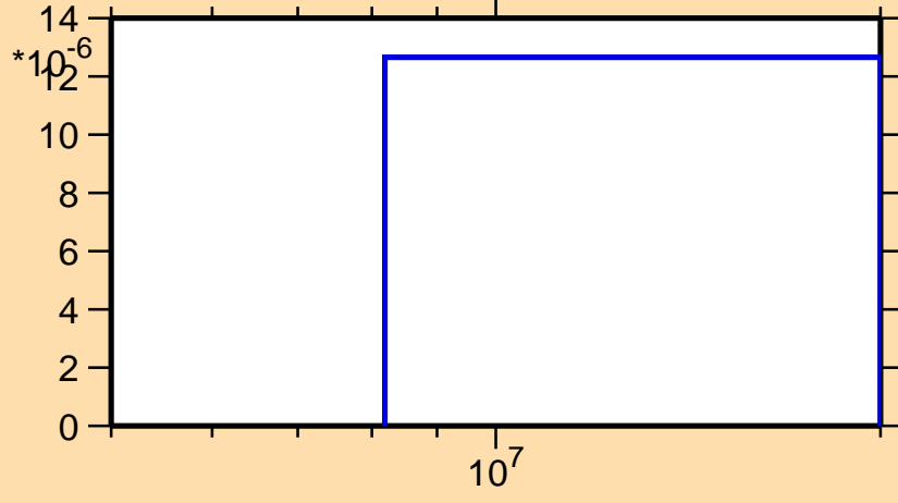
\sigma vs. E for ^{111}\text{I}(n,\text{pt})
