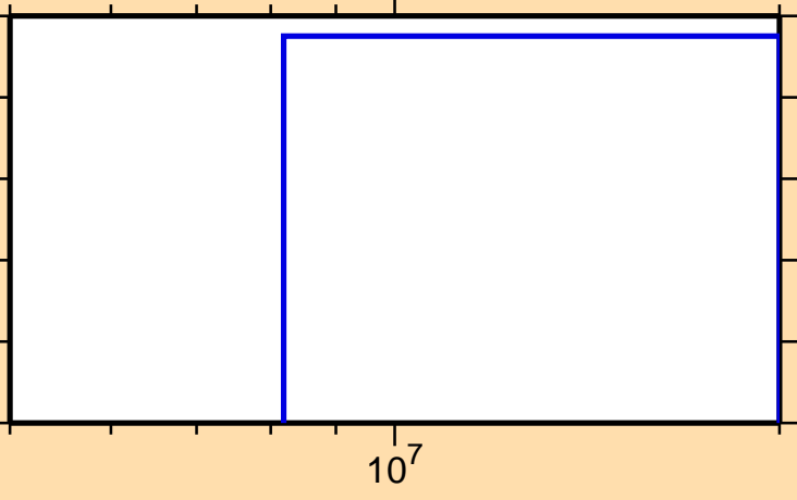
\sigma vs. E for ^{111}\text{I}(n,\text{nd})
