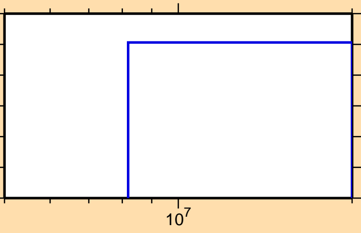
\sigma vs. E for ^{111}\text{I}(n,2np)
