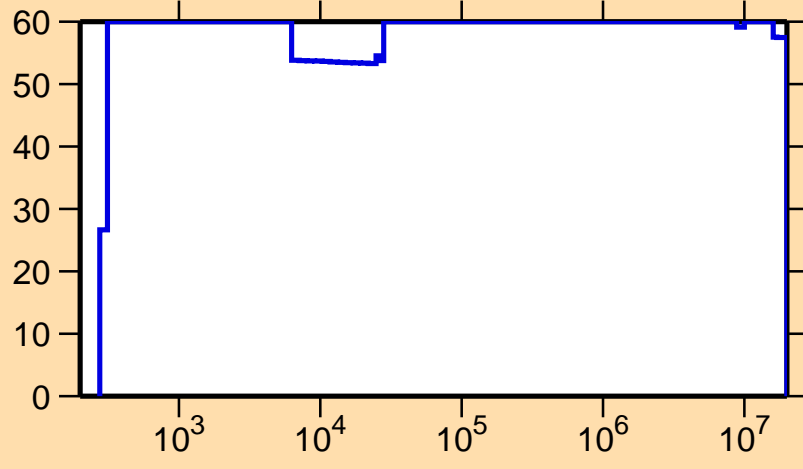
\Delta\sigma/\sigma vs. E for ^{112}\text{I}(n,p)
