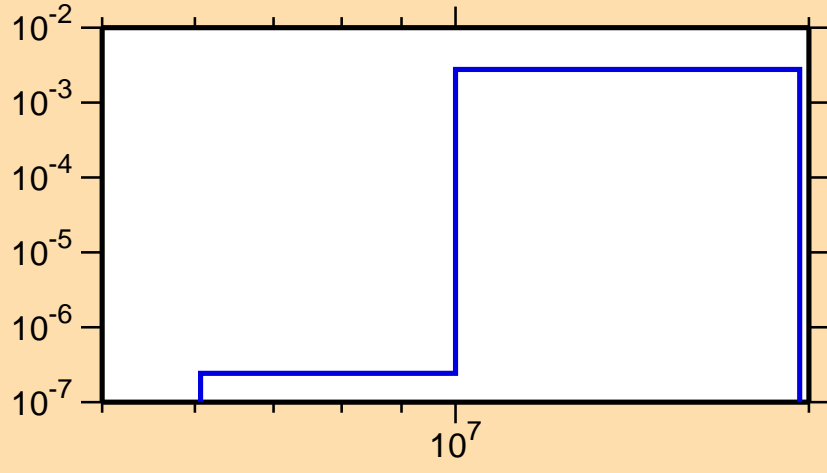
\sigma vs. E for ^{112}\text{I}(n,p,d)
