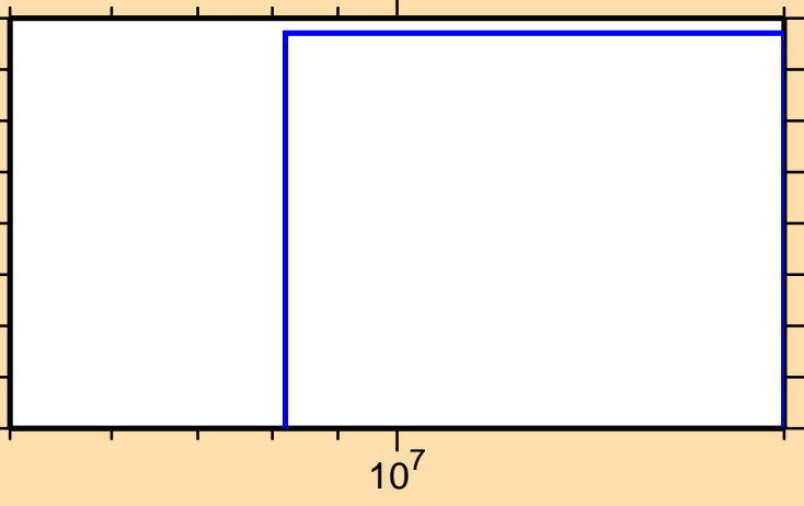
\sigma vs. E for ^{112}\text{I}(n,\text{nd})
