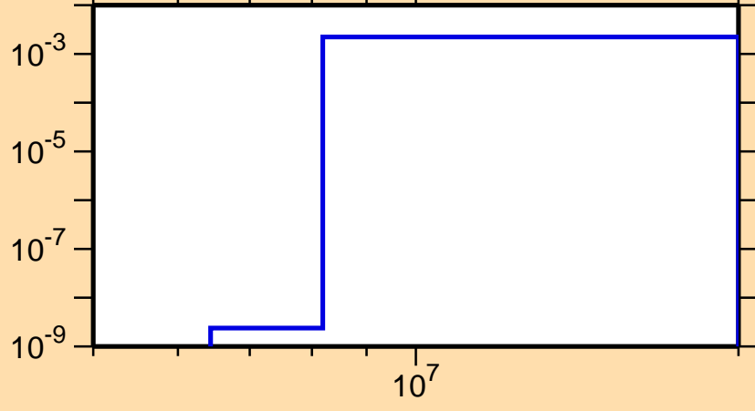
\sigma vs. E for ^{112}\text{I}(n,\text{pd})
