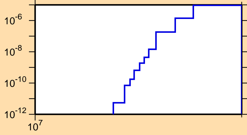
\sigma vs. E for ^{113}\text{I}(n,\text{nd})
