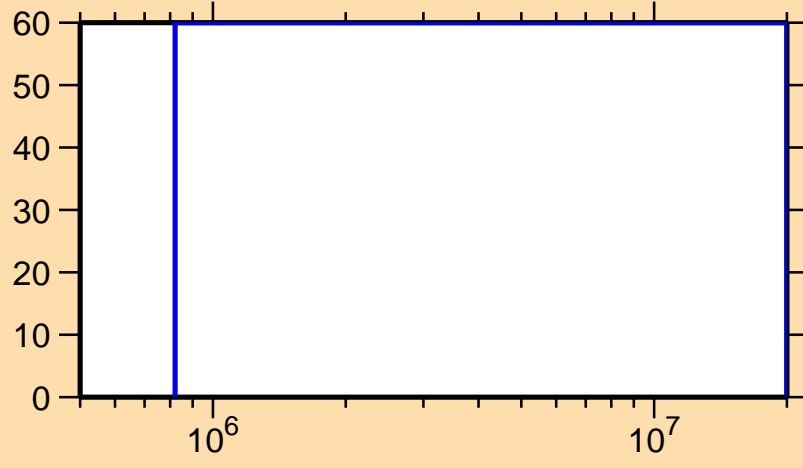
\Delta\sigma/\sigma vs. E for ^{113}\text{I}(n,n\text{cont.})
