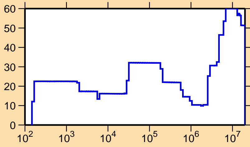
\Delta\sigma/\sigma vs. E for ^{113}\text{I}(n,p)
