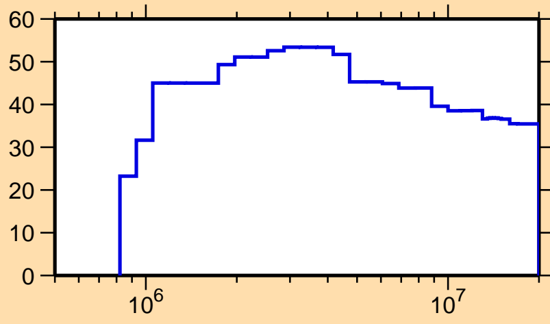
\Delta\sigma/\sigma vs. E for ^{113}\text{I}(n,n_1)
