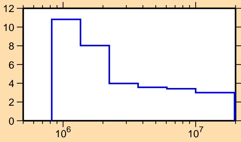
\Delta\sigma/\sigma vs. E for ^{113}\text{I}(n, nonel.)
