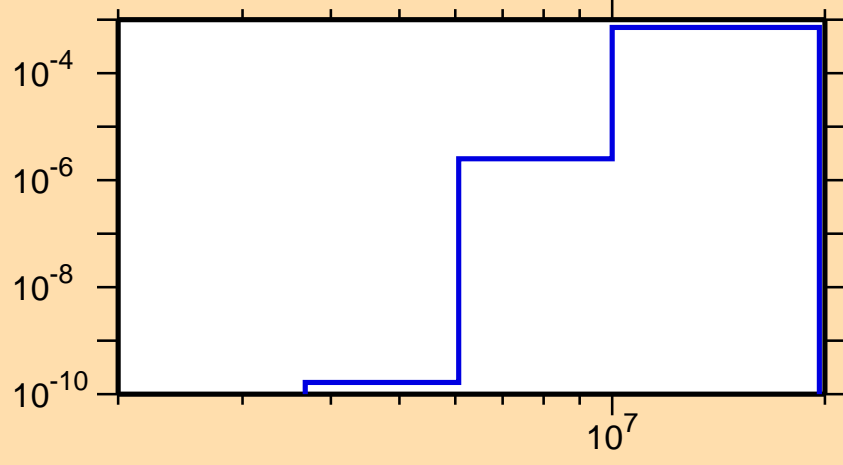
\sigma vs. E for ^{113}\text{I}(\text{mt117})
