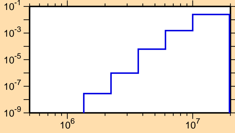
\sigma vs. E for ^{113}\text{I}(n,d)
