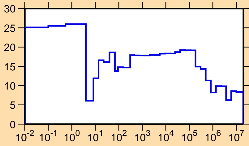
\Delta\sigma/\sigma vs. E for ^{113}\text{I}(n,\text{el.})
