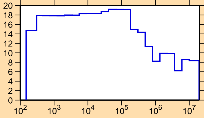
\Delta\sigma/\sigma vs. E for ^{113}\text{I}(n,\text{el.})
