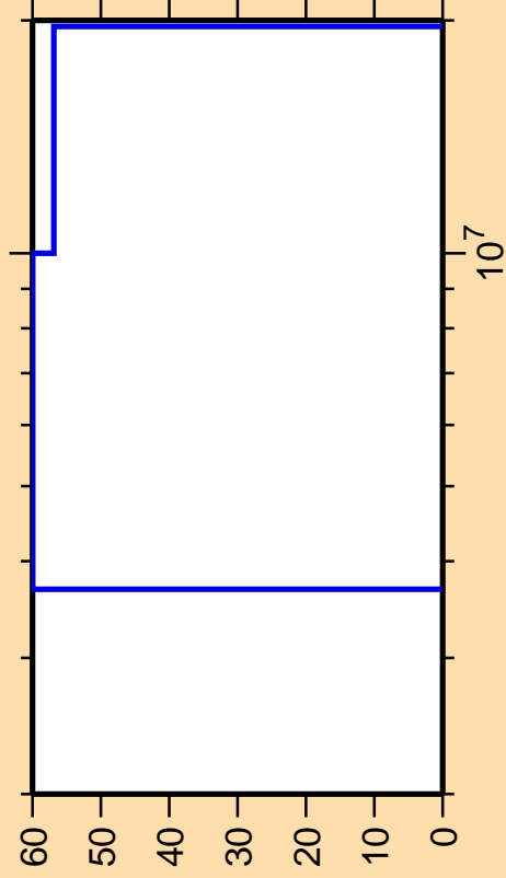
\Delta\sigma/\sigma vs. E for ^{113}\text{I} (mt 45)
