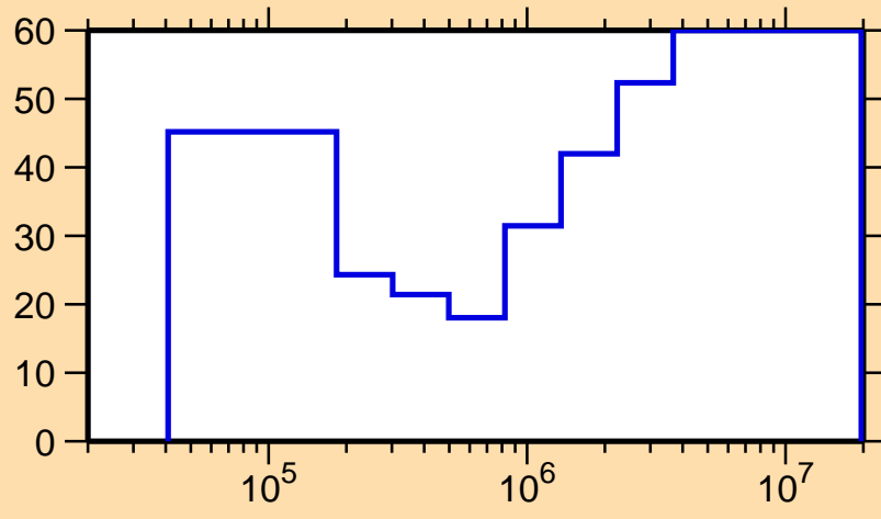
\Delta\sigma/\sigma vs. E for ^{113}\text{I}(n,\text{inel.})
