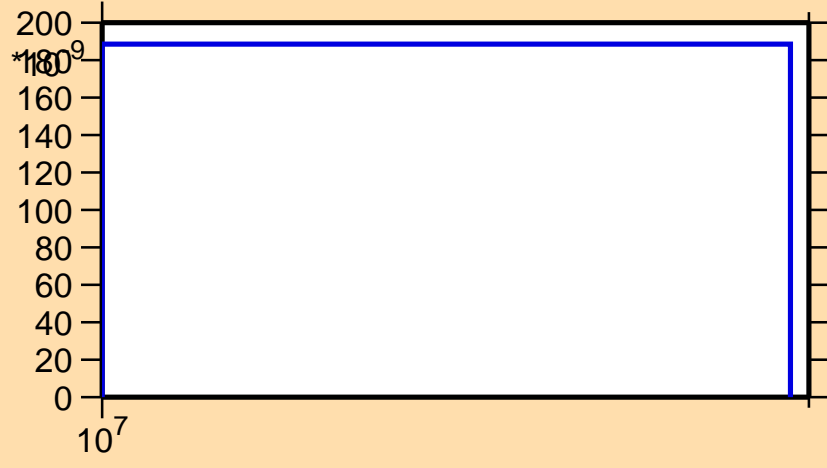
\sigma vs. E for ^{113}\text{I}(n,nd)
