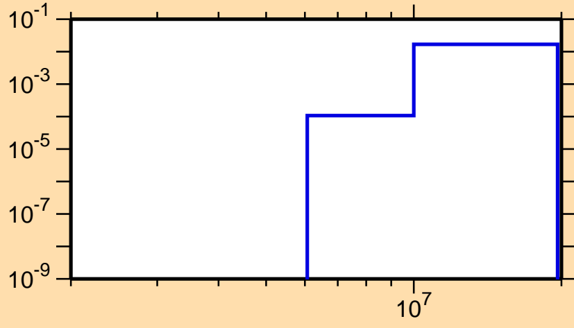
\sigma vs. E for ^{113}\text{I} (mt 45)
