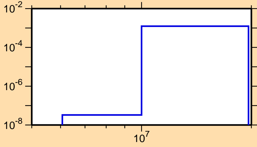
\sigma vs. E for ^{113}\text{I}(n,\text{pd})
