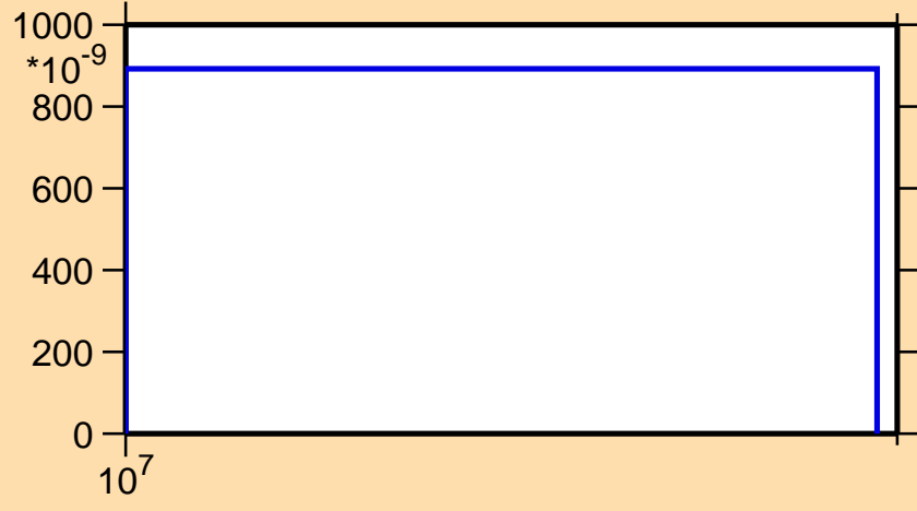
\sigma vs. E for ^{113}\text{I}(n,\text{pt})
