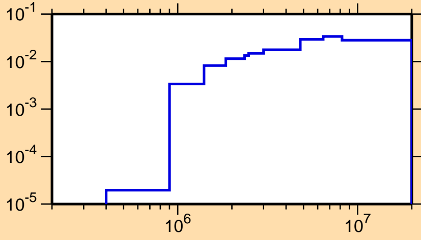
\sigma vs. E for ^{113}\text{I}(n,n\text{cont.})
