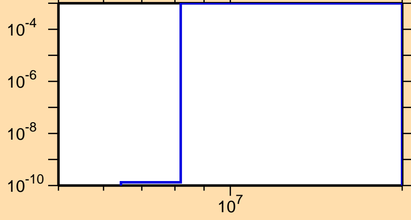
\sigma vs. E for ^{113}\text{I}(n,\text{pd})
