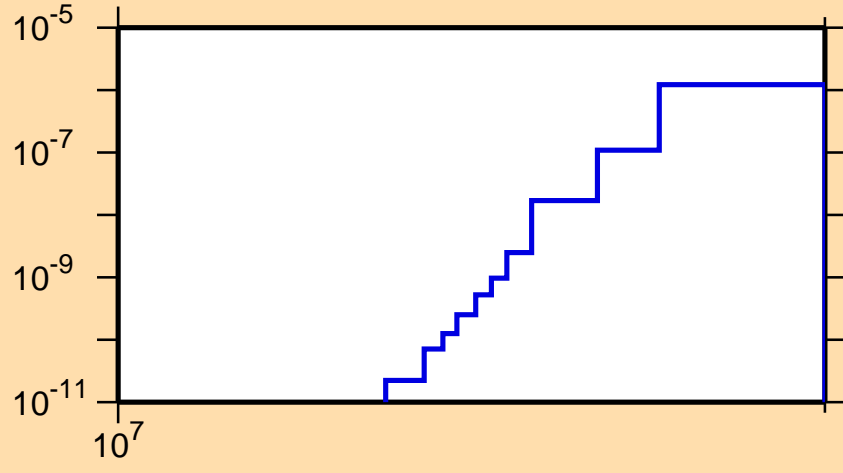
\sigma vs. E for ^{114}\text{I} (mt 34)
