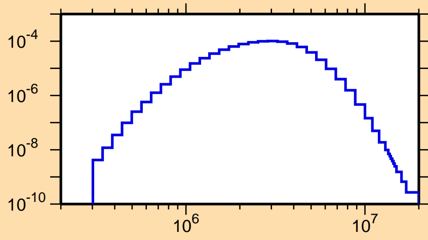
\sigma vs. E for ^{114}\text{I}(n,n_3)
