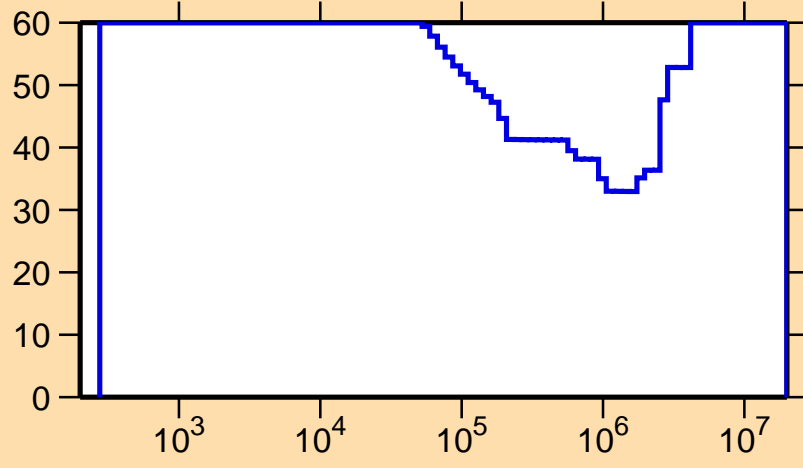
\Delta\sigma/\sigma vs. E for ^{114}\text{I}(n,p)
