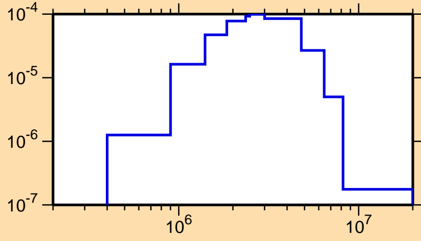
\sigma vs. E for ^{114}\text{I}(n,n_3)
