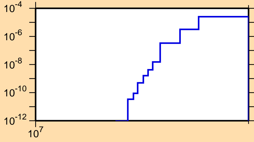
\sigma vs. E for ^{115}\text{I}(n,\text{nd})
