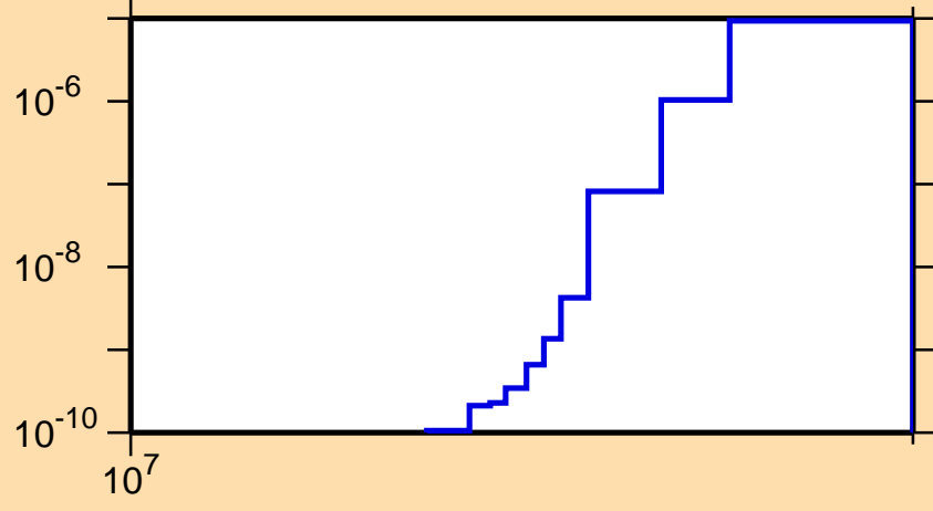
\sigma vs. E for ^{115}\text{I}(n,2n\alpha)
