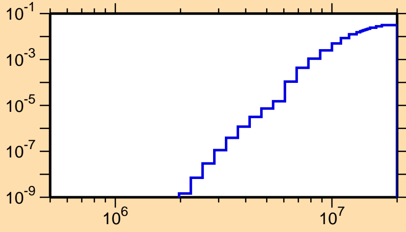
\sigma vs. E for ^{115}\text{I}(n,d)
