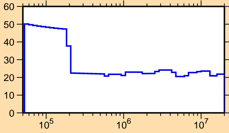
\Delta\sigma/\sigma vs. E for ^{115}\text{I}(n,\text{nonel.})
