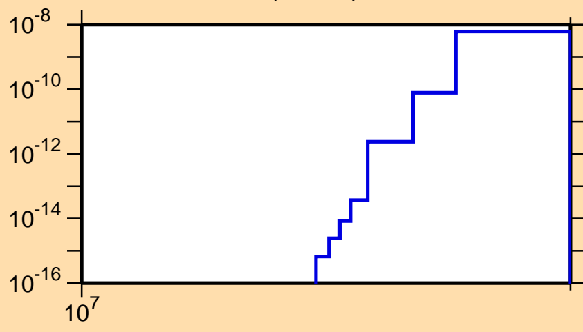
\sigma vs. E for ^{115}\text{I} (mt 34)
