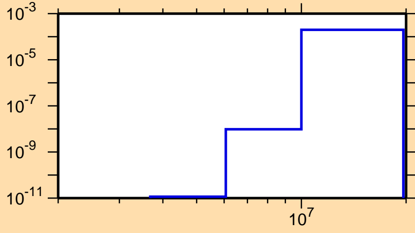
\sigma vs. E for ^{115}\text{I}(n,\text{He}3)
