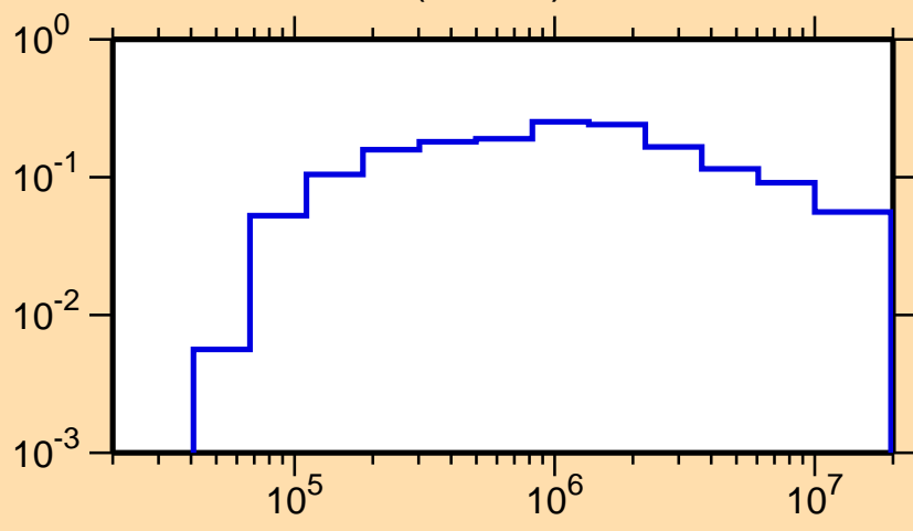
\sigma vs. E for ^{115}\text{I}(n,\text{inel.})
