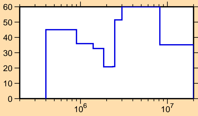
\Delta\sigma/\sigma vs. E for ^{115}\text{I}(n, el.)
