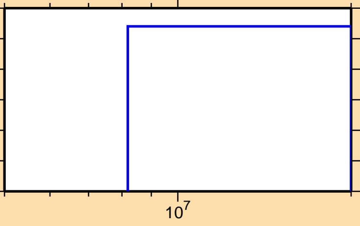
\sigma vs. E for ^{115}\text{I}(n,2n)
