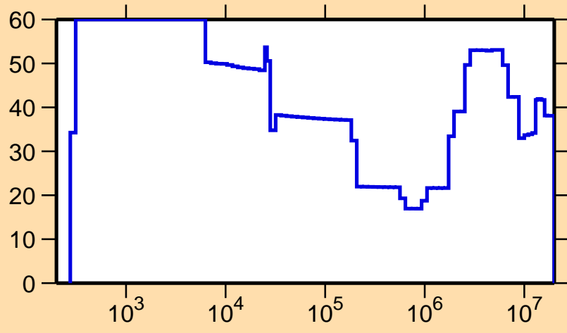
\Delta\sigma/\sigma vs. E for ^{116}\text{I}(n,p)
