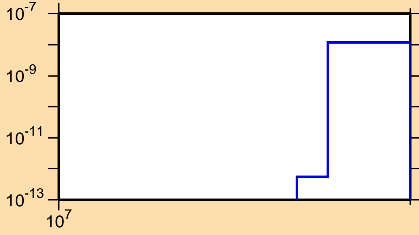
\sigma vs. E for ^{116}\text{I}(n,nt)
