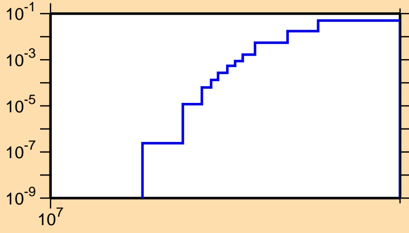
\sigma vs. E for ^{116}\text{I}(n,2np)
