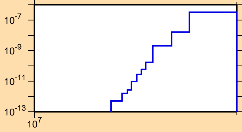
\sigma vs. E for ^{116}\text{I} (mt 34)
