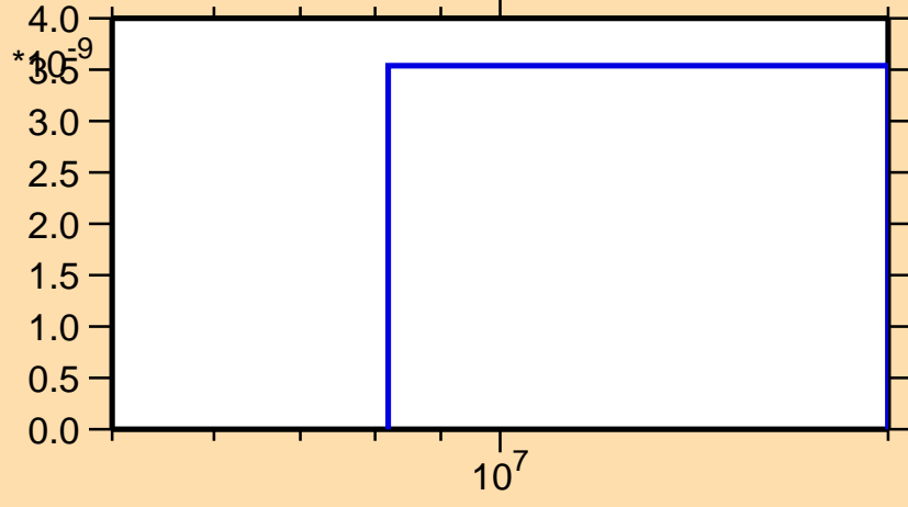
\sigma vs. E for ^{116}\text{I}(\text{mt } 34)
