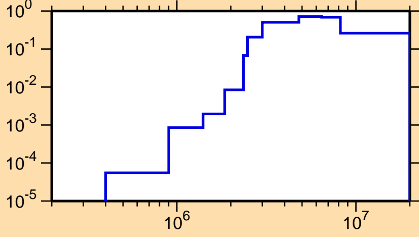
\sigma vs. E for ^{116}\text{I}(n,n\text{cont.})
