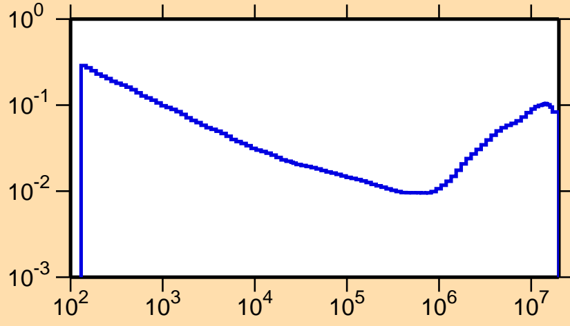
\sigma vs. E for ^{117}\text{I}(n,\alpha)
