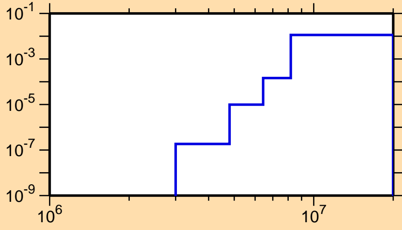
\sigma vs. E for ^{117}\text{I}(n,d)
