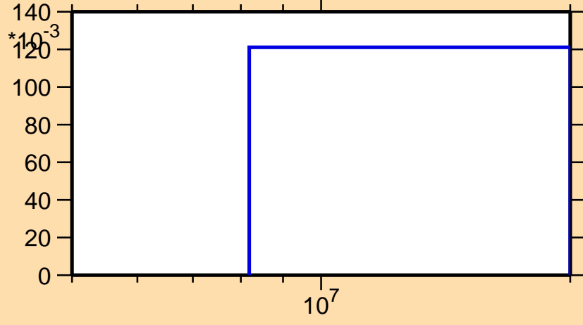
\sigma vs. E for ^{117}\text{I}(n,2n)
