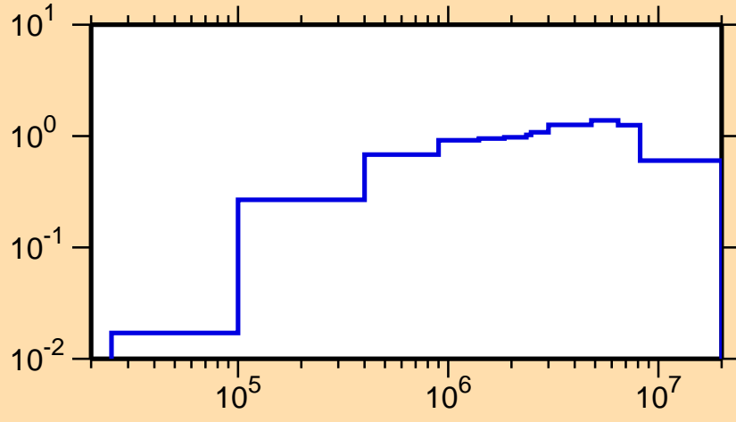
\sigma vs. E for ^{117}\text{I}(n,\text{inel.})
