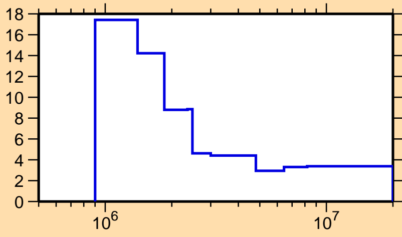
\Delta\sigma/\sigma vs. E for ^{117}\text{I}(n, nonel.)
