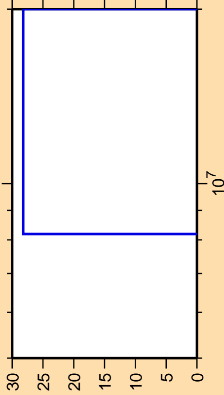
\Delta\sigma/\sigma vs. E for ^{117}\text{I}(n,p)
