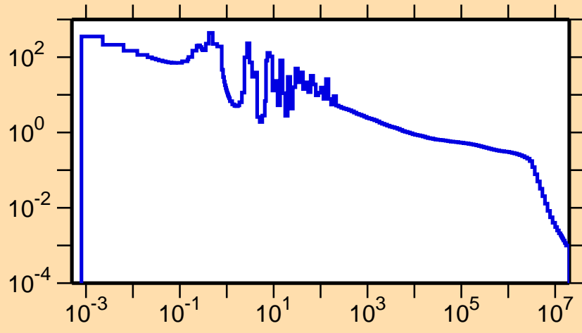
\sigma vs. E for ^{118}\text{I}(n,\gamma)
