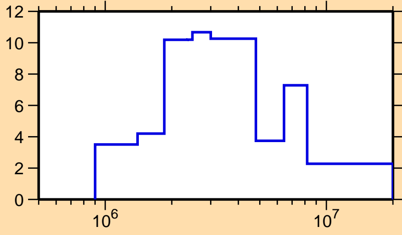
\Delta\sigma/\sigma vs. E for ^{118}\text{I}(n, el.)
