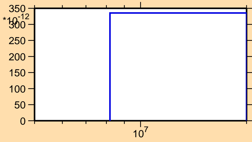
\sigma vs. E for ^{118}\text{I}(\text{mt } 34)
