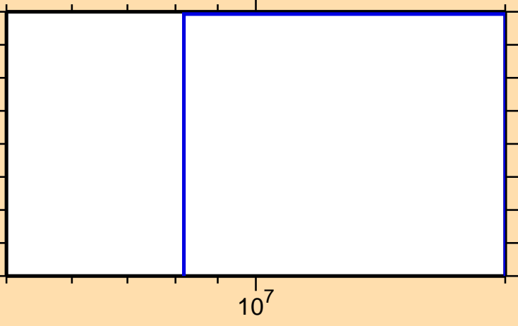
\sigma vs. E for ^{118}\text{I}(\text{mt117})
