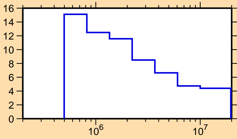
\Delta\sigma/\sigma vs. E for ^{118}\text{I}(n, n\text{onrel.})
