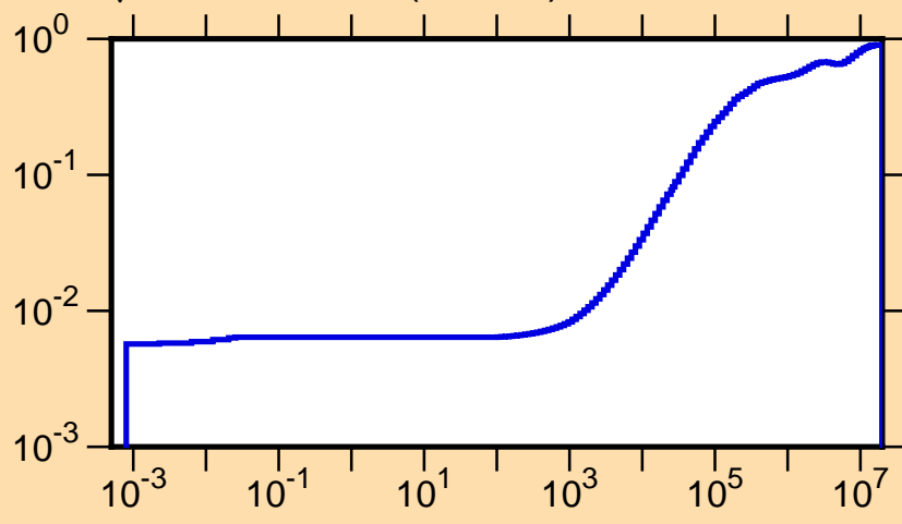
\mu vs. E for ^{119}\text{I}(\text{mt251})
