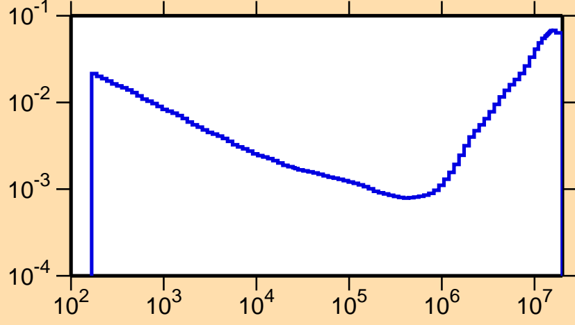
\sigma vs. E for ^{119}\text{I}(n,\alpha)
