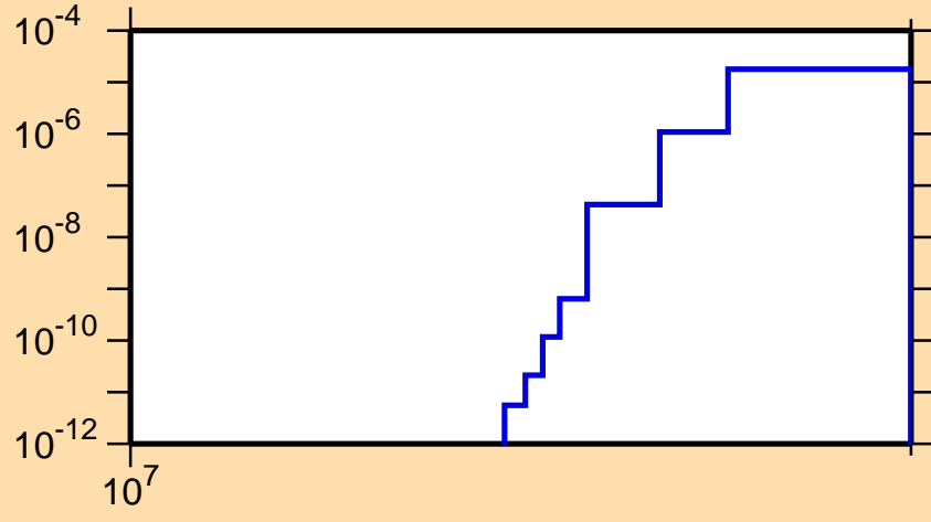
\sigma vs. E for ^{119}\text{I}(n,\text{nd})
