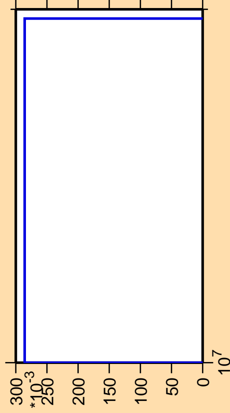
\Delta\sigma/\sigma vs. E for ^{119}\text{I}(n,3n)
