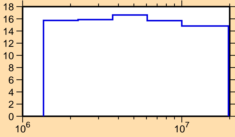
\Delta\sigma/\sigma vs. E for ^{119}\text{I}(n, nonel.)
