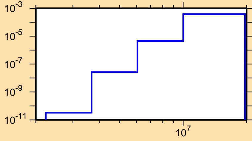
\sigma vs. E for ^{119}\text{I}(n,p\alpha)
