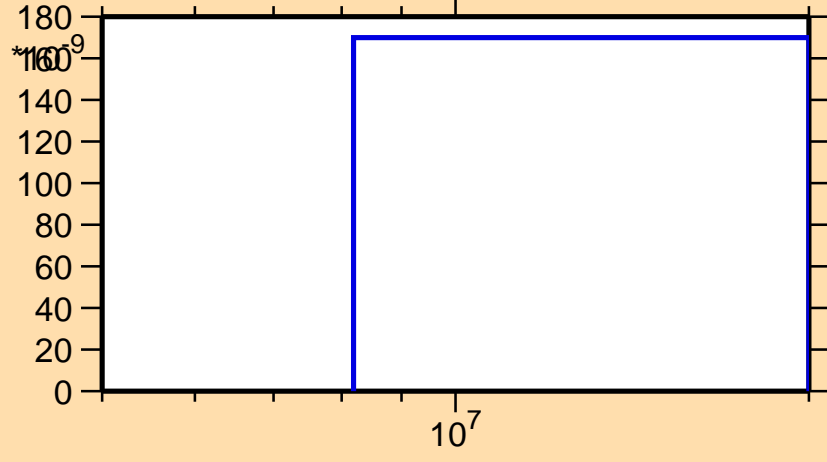
\sigma vs. E for ^{119}\text{I}(n,2n\alpha)
