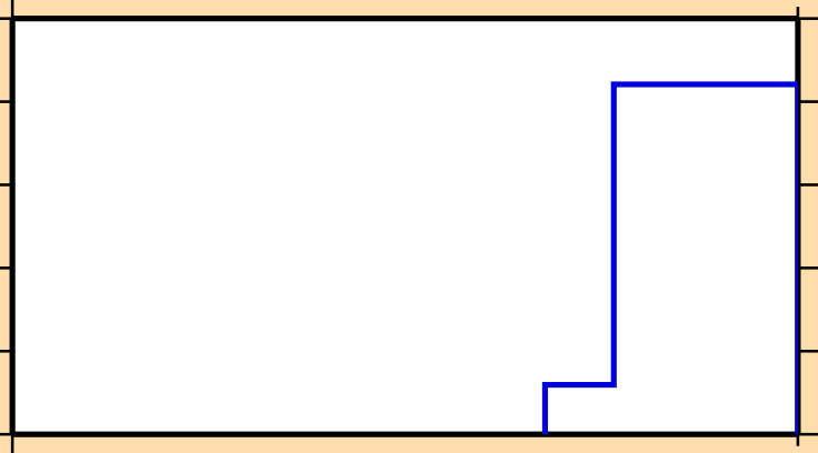
\sigma vs. E for ^{120}\text{I}(n,nt)
