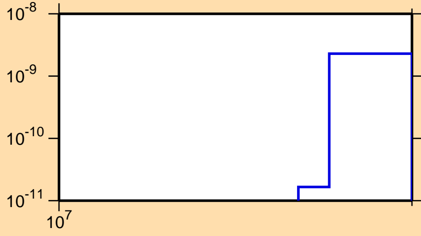
\sigma vs. E for ^{120}\text{I} (mt 34)
