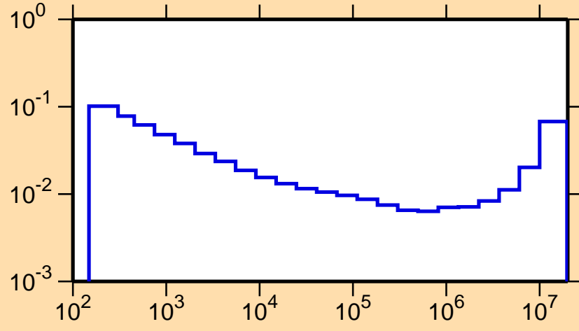
\sigma vs. E for ^{120}\text{I}(n,\alpha)
