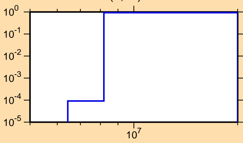
\sigma vs. E for ^{120}\text{I}(n,2n)
