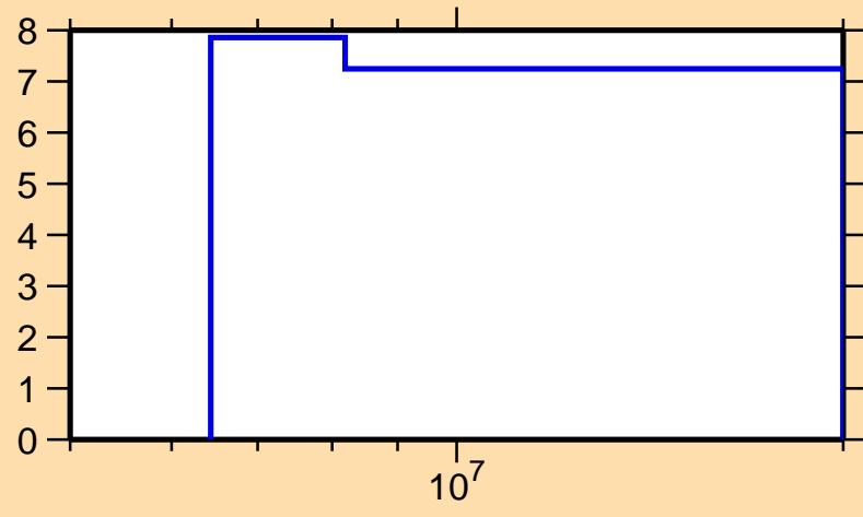
\Delta\sigma/\sigma vs. E for ^{120}\text{I}(n,\text{nonel.})
