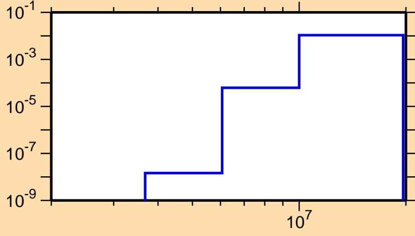
\sigma vs. E for ^{120}\text{I}(n,d)
