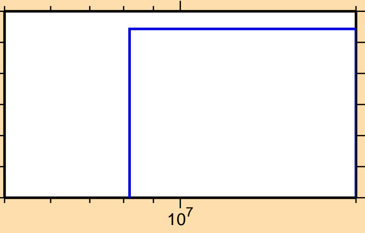
\sigma vs. E for ^{120}\text{I}(n,\text{He3})
