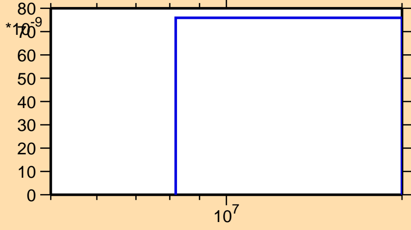
\sigma vs. E for ^{120}\text{I}(n,3n)
