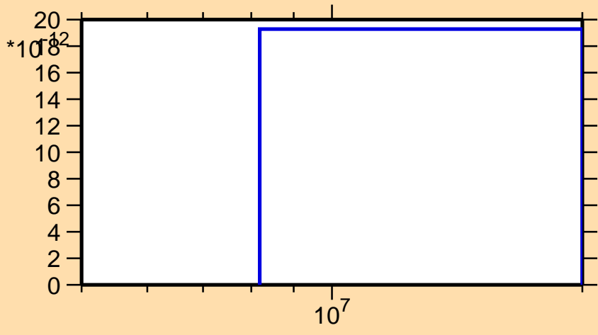
\sigma vs. E for ^{120}\text{I}(\text{mt } 34)
