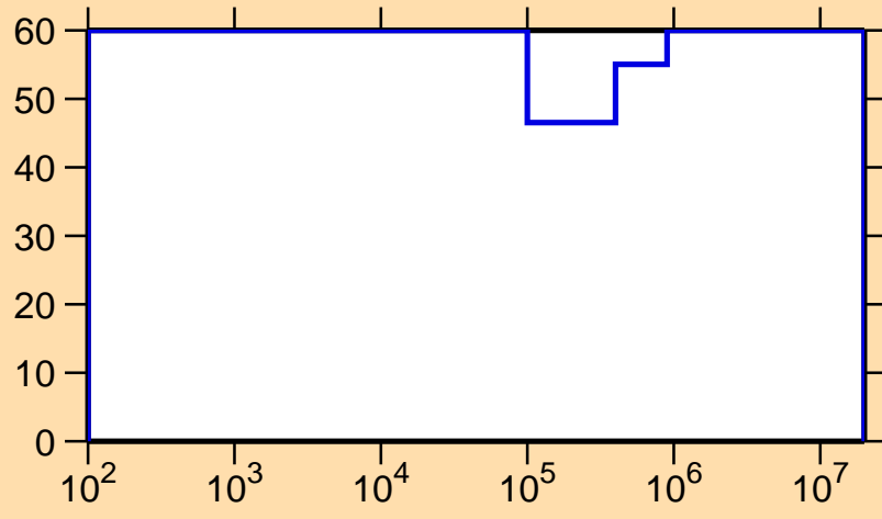
\Delta\sigma/\sigma vs. E for ^{120}\text{I}(n,\gamma)
