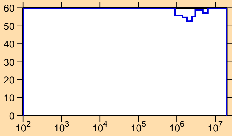
\Delta\sigma/\sigma vs. E for ^{120}\text{I}(n,n_1)
