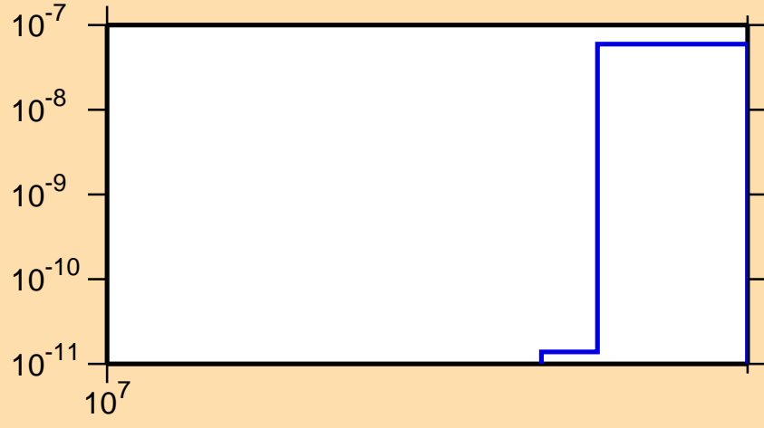
\sigma vs. E for ^{121}\text{I}(n,nt)
