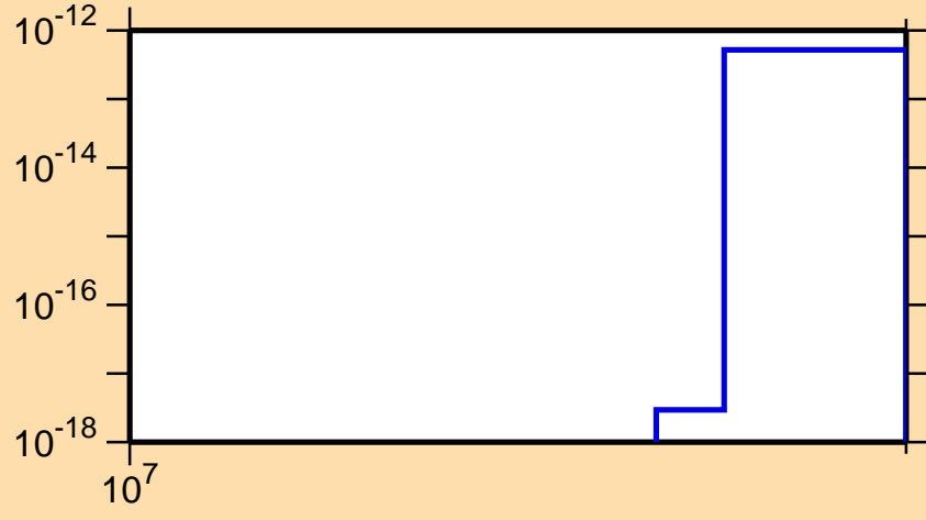
\sigma vs. E for ^{121}\text{I}(n,\text{pt})
