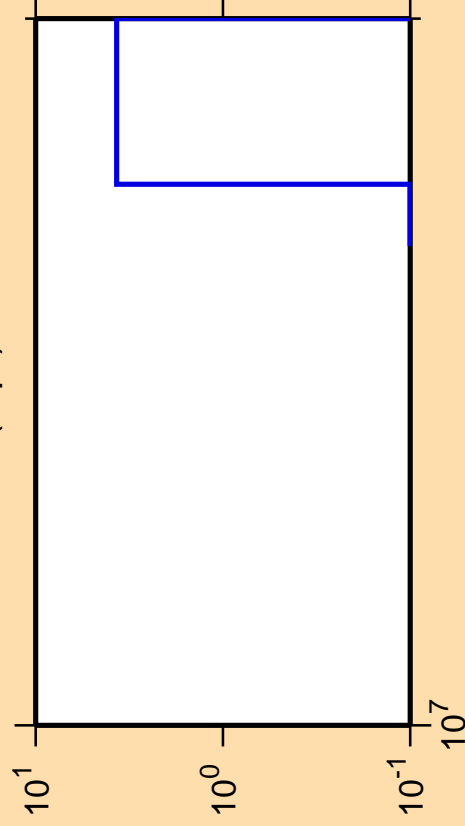
\Delta\sigma/\sigma vs. E for ^{121}\text{I}(n,\text{pt})
