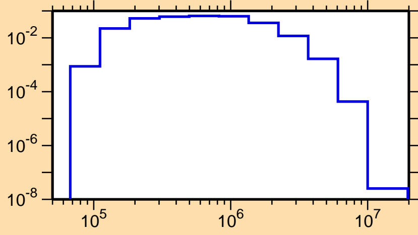
\sigma vs. E for ^{121}\text{I}(n,n_1)
