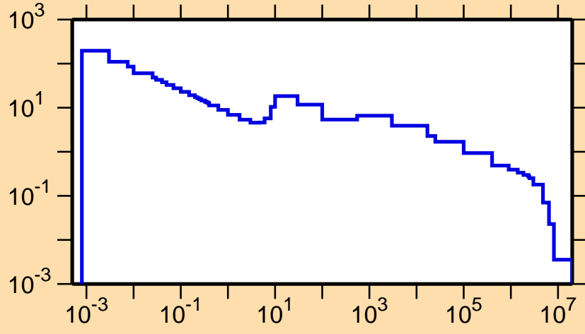
\sigma vs. E for ^{121}\text{I}(n,\gamma)
