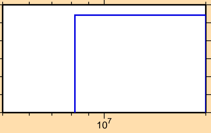
\sigma vs. E for ^{121}\text{I} (mt 45)
