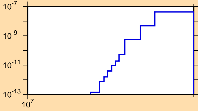
\sigma vs. E for ^{122}\text{I} (mt 45)
