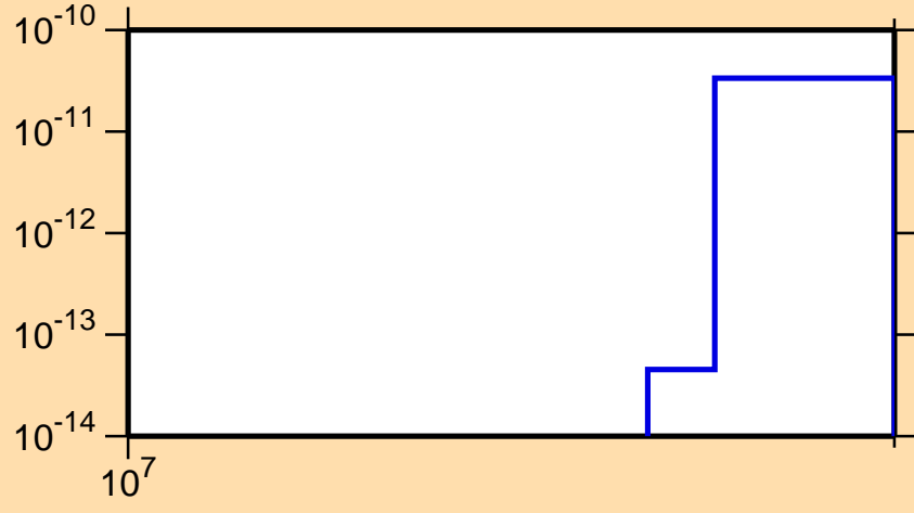
\sigma vs. E for ^{122}\text{I} (mt 34)
