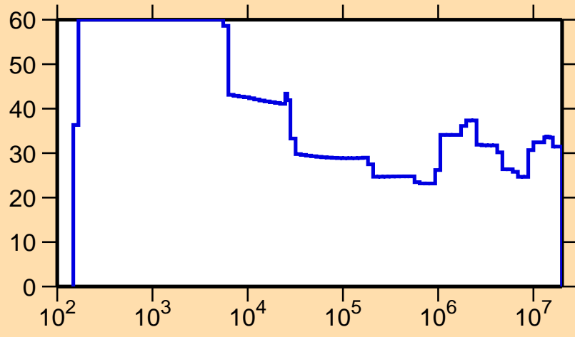
\Delta\sigma/\sigma vs. E for ^{122}\text{I}(n,p)
