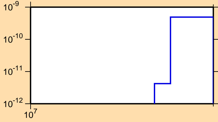
\sigma vs. E for ^{122}\text{I}(n,\text{pd})
