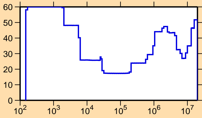
\Delta\sigma/\sigma vs. E for ^{122}\text{I}(n,\gamma)
