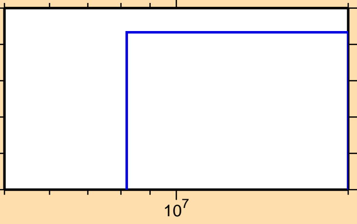
\sigma vs. E for ^{122}\text{I}(n,\text{He}3)
