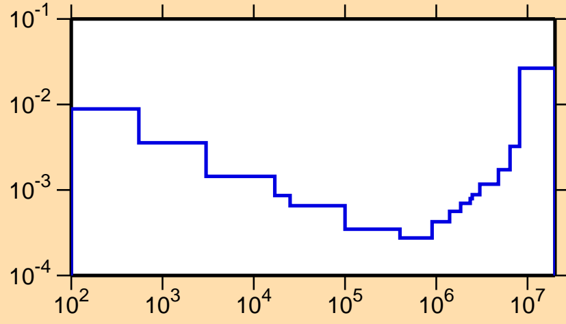
\sigma vs. E for ^{122}\text{I}(n,\alpha)
