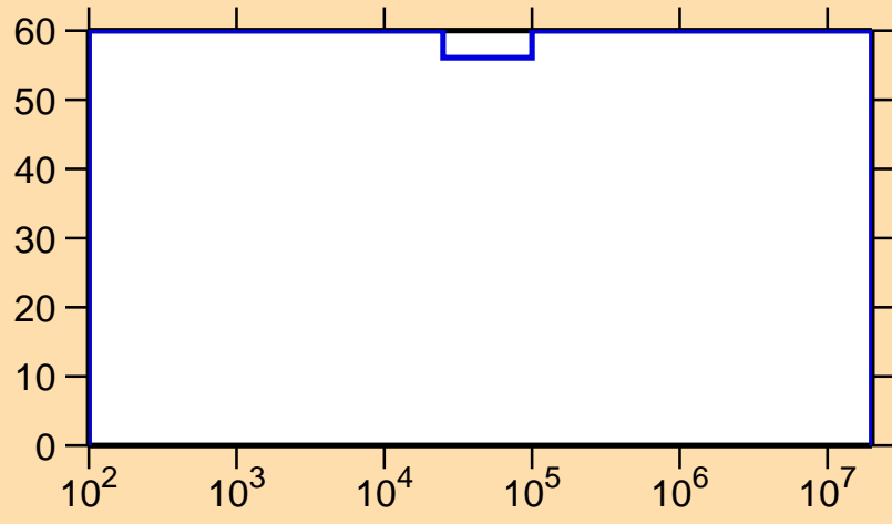
\Delta\sigma/\sigma vs. E for ^{123}\text{I}(n,\gamma)
