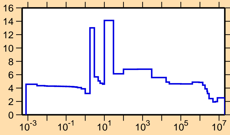
\sigma vs. E for ^{123}\text{I}(n,\text{el.})
