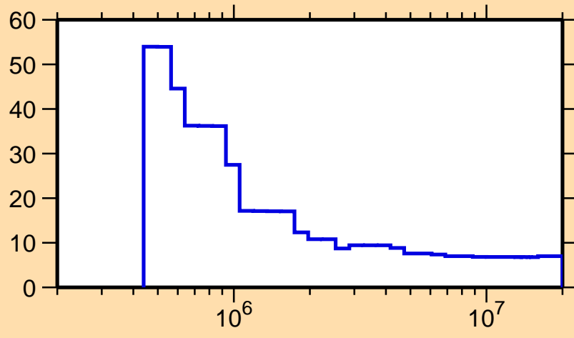
\Delta\sigma/\sigma vs. E for ^{124}\text{I}(n, nonel.)
