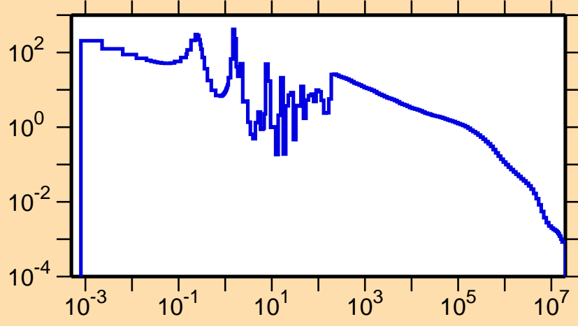
\sigma vs. E for ^{124}\text{I}(n,\gamma)
