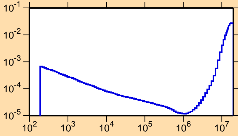
\sigma vs. E for ^{124}\text{I}(n,\alpha)
