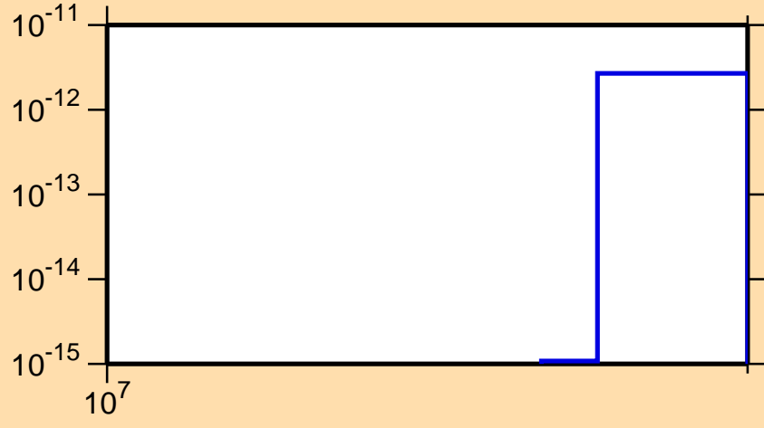
\sigma vs. E for ^{124}\text{I}(n,\text{pd})
