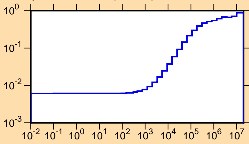
\mu vs. E for ^{124}\text{I} (mt251)
