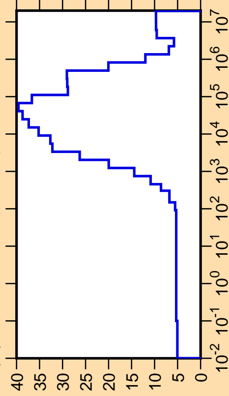
\Delta\mu/\mu vs. E for ^{124}\text{I} (mt251)
