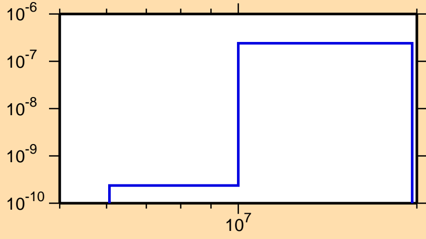
\sigma vs. E for ^{124}\text{I}(n,p\alpha)
