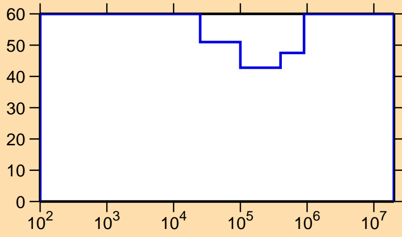
\Delta\sigma/\sigma vs. E for ^{124}\text{I}(n,\gamma)
