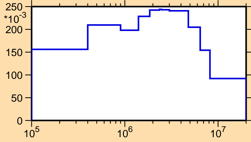
\sigma vs. E for ^{124}\text{I}(n,n_2)
