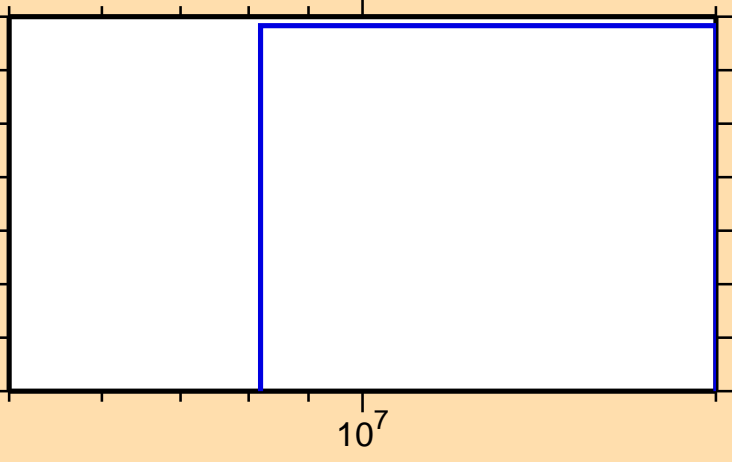
\sigma vs. E for ^{124}\text{I}(\text{mt117})
