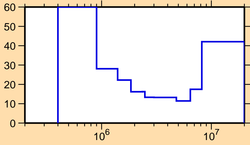
\Delta\sigma/\sigma vs. E for ^{124}\text{I}(n,ncont.)
