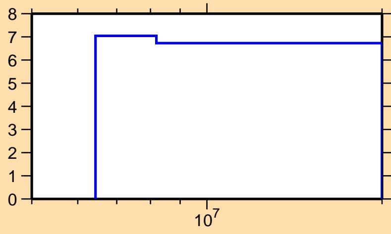
\Delta\sigma/\sigma vs. E for ^{124}\text{I}(n,\text{nonel.})
