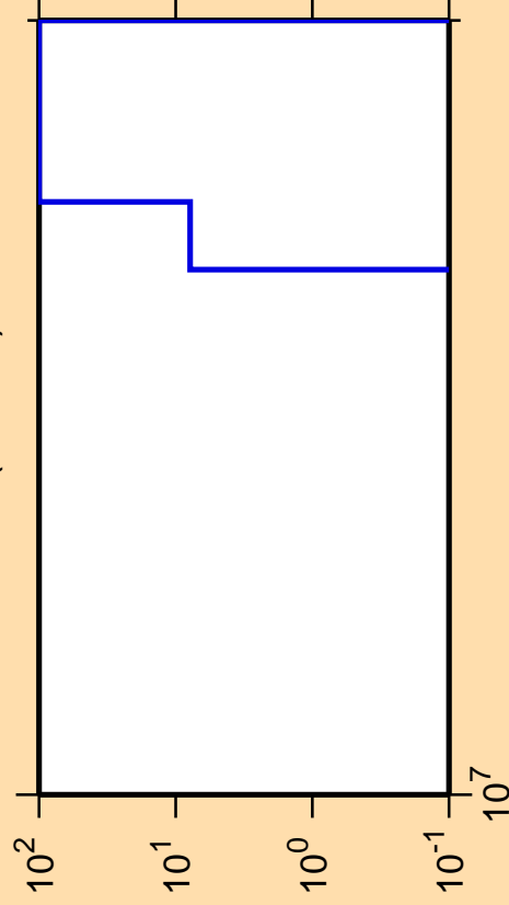
\Delta\sigma/\sigma vs. E for ^{125}\text{I} (mt117)
