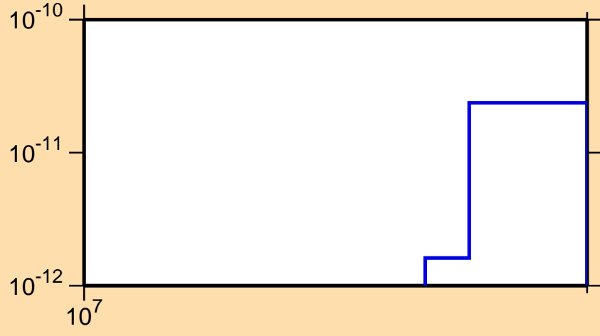
\sigma vs. E for ^{125}\text{I} (mt117)
