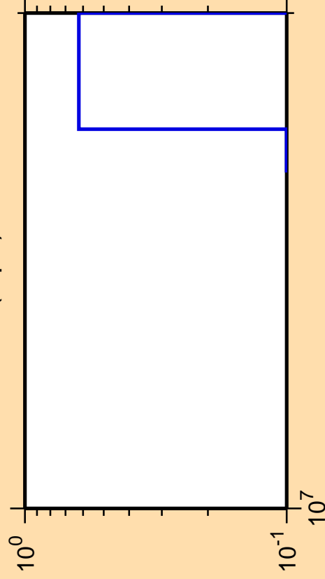
\Delta\sigma/\sigma vs. E for ^{125}\text{I}(n,\text{pd})
