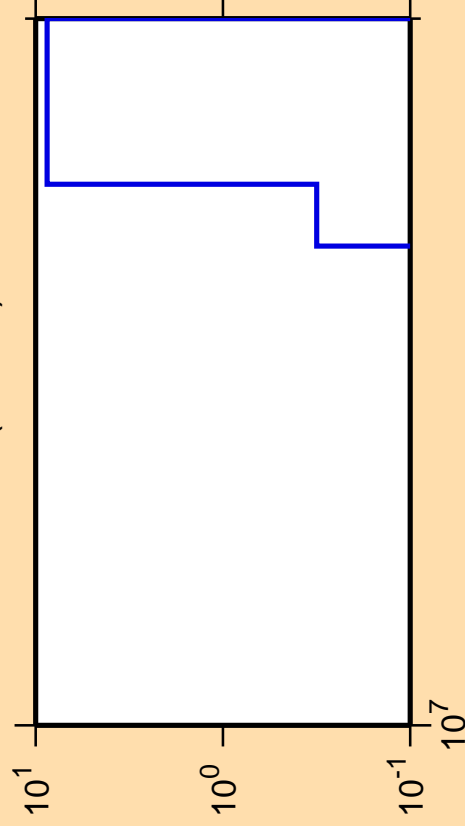
\Delta\sigma/\sigma vs. E for ^{126}\text{I}(\text{mt117})
