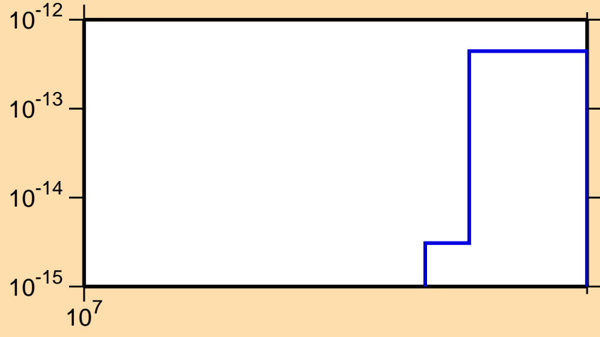
\sigma vs. E for ^{126}\text{I} (mt 45)
