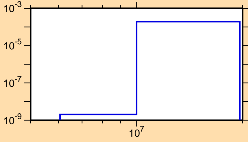
\sigma vs. E for ^{126}\text{I}(n,t)
