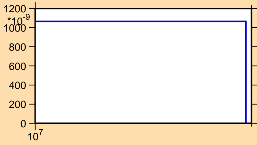
\sigma vs. E for ^{126}\text{I}(n,\text{nd})
