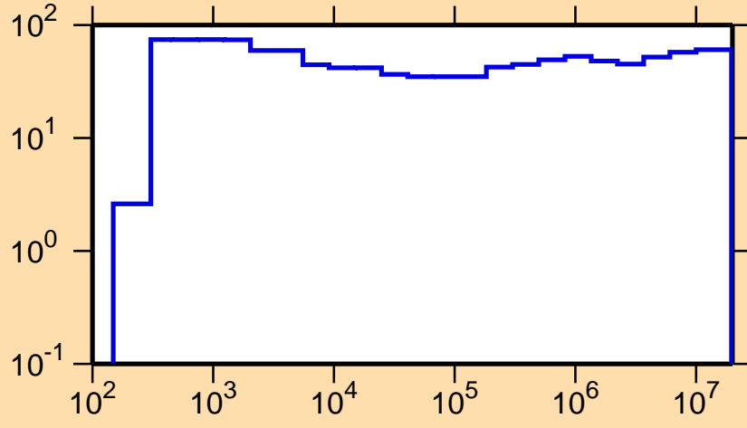
\Delta\sigma/\sigma vs. E for ^{126}\text{I}(n,p)
