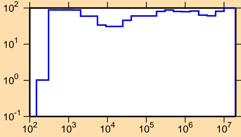
\Delta\sigma/\sigma vs. E for ^{126}\text{I}(n,\gamma)
